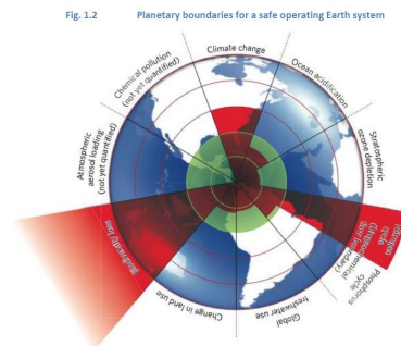
Fig. 1.2 Planetary boundaries for a safe operating Earth system
